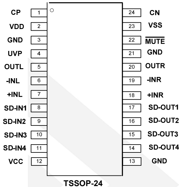
Figure 1 Pin Assignment
